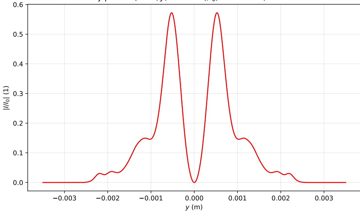
Intensity profile I(x=0, y, z=2.707)/I_0 , P_{in}=5.0P_{cr} , artificial time
